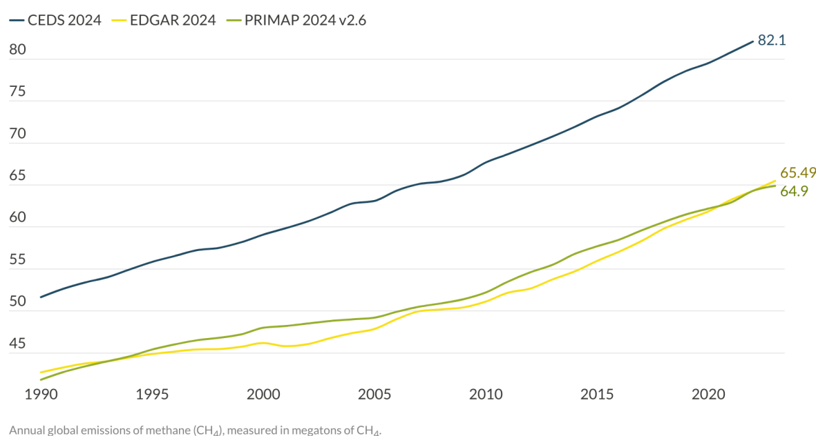
Figure 6: Historic trends in global methane emissions in the waste sector
