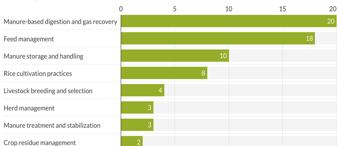
Figure 12c: Mitigation types in the Agriculture Sector
