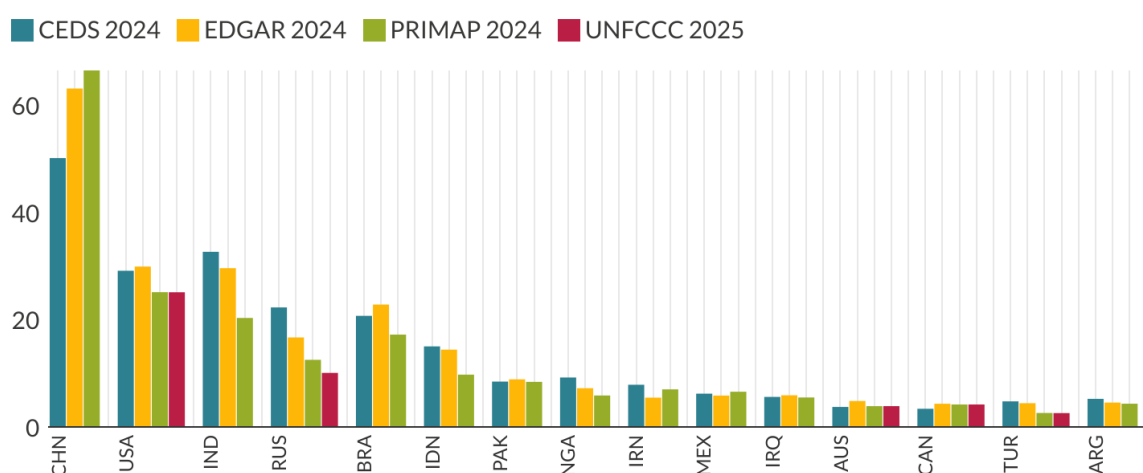
Figure 10: Comparison of methane emissions for top emitters across datasets (2022)
