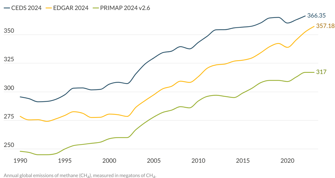
Figure 1: Historic trends in global methane emissions
