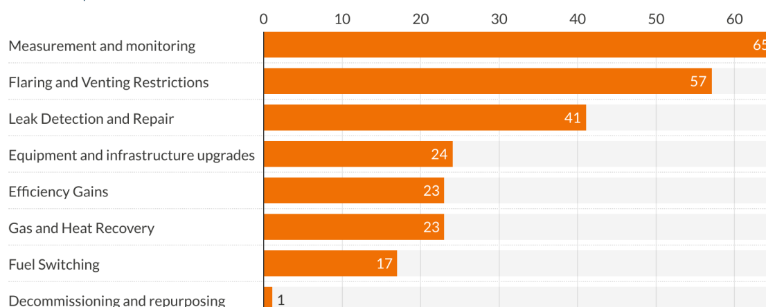
Figure 12a: Mitigation types in the Energy Sector
