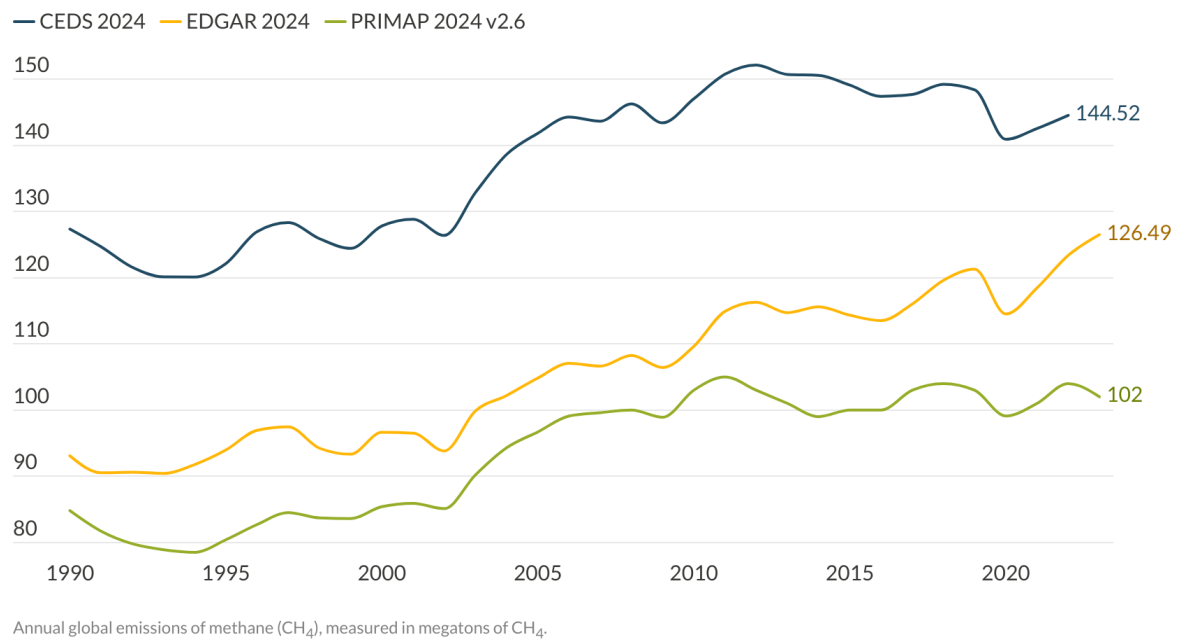
Figure 5: Historic trends in global methane emissions in the energy sector
