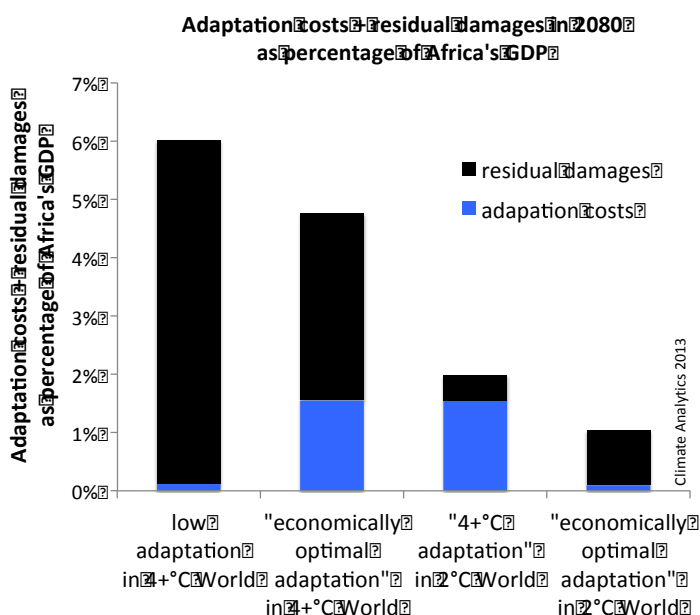
Figure ES.1. Overview of adaptation costs and residual damages for Africa (excl. those related to sea-level rise) in relation to two mitigation scenarios and various adaptation cases. Both higher warming and low adaptation lead to rapidly increasing residual damages. “Economically optimal” is the level of adaptation that results in the lowest total of adaptation costs and residual damages over the whole of the 21 st century. “4+°C adaptation” signifies a level of adaptation equal to “economic adaptation” in a 4+°C world that leads to strongly reduced damages in a 2°C world
