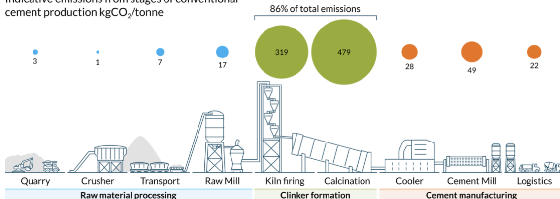
Figure 1: Indicative emissions from the conventional cement production process, adapted from Czigler et al. (2020). 5
